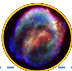
SUPERNOVA
