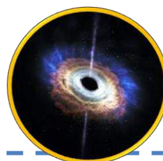
BLACK HOLE
