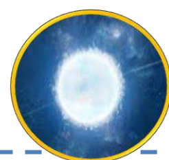
WHITE DWARF
