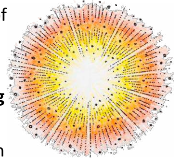
The big bang
